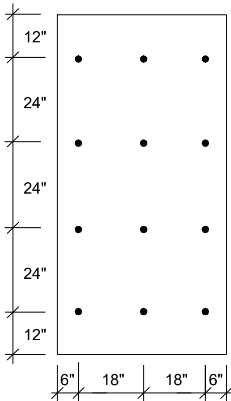
12 FASTENERS PER 4' x 8' BOARD
