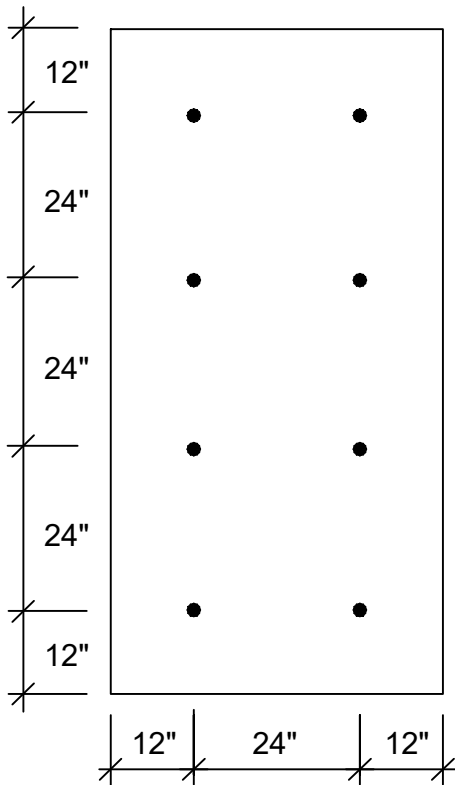
8 FASTENERS PER 4' x 8' BOARD
